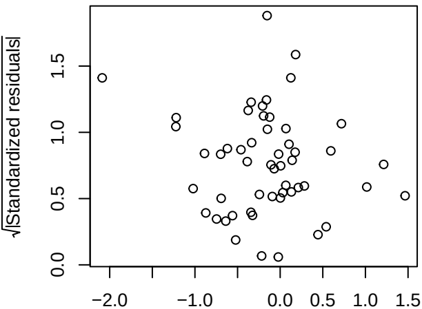
Scale-Location
